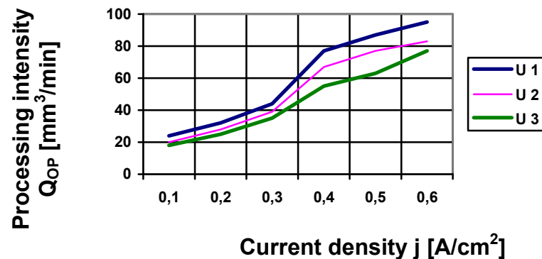
Figure 8: The influence of the j current density on the productivity of the Q_{OP} processing for the values of the voltage U_1 = 28 V; U_2 = 24 V; U_3 = 20 V.
