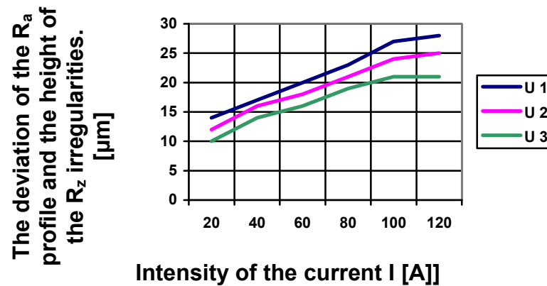
Figure 7: The influence of the I current intensity on the R_z irregularities height for the values of the voltage: U_1 = 28 V; U_2 = 24 V; U_3 = 20 V.
