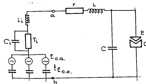
Fig 4 Capacitive circuit
